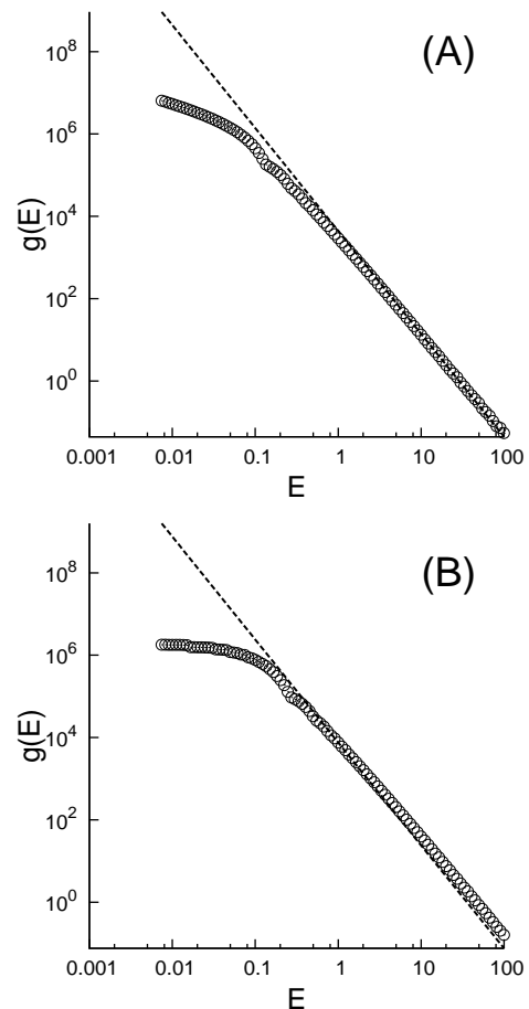
FIG. 28 Simulation results for g(E) characterizing energy bursts in fiber bundles with (A) the uniform threshold distribution (Eq. 1) and (B) the Weibull distribution (Eq. 2) of index 2. The graphs are based on 1000 samples with N = 10^6 fibers in each bundle. Open circles represent simulation data, and dashed lines are the theoretical results (Eqs. 226 - 227) for the asymptotics.
