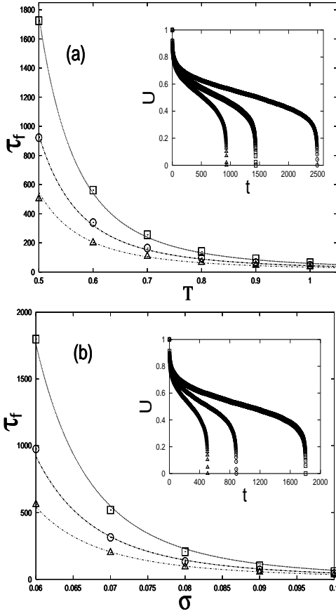
FIG. 48 Simulation results of fatigue behavior: (a) average failure time \tau_f vs. noise T ( K = 1 here) for three different stress values and (b) \tau_f vs. \sigma for three different noise values. The bundle contains N = 10^5 fibers with uniformly distributed strength thresholds. The time variations of fraction of surviving fibers are shown in the insets. The dotted lines in (a) and (b) correspond to the fit with expression (Eq. 278) where \sigma_c \simeq 0.245 (exact value=1/4 (Bhattacharyya et al. , 2003; Pradhan et al. , 2002)).
