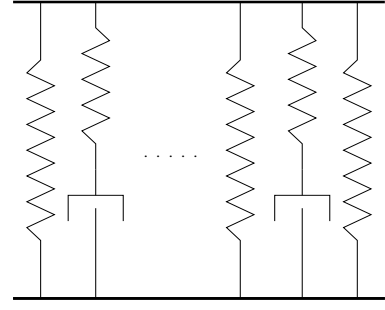
FIG. 51 The fibers are modeled by Maxwell elements. From Kun et al. (2003)
