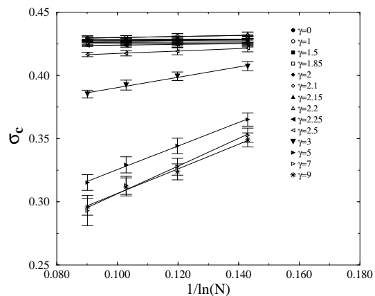
FIG. 36 Strength at failure, \sigma_c as a function of the number of fibers N for different range exponents \gamma in the variable range fiber bundle of Hidalgo et al. (2002).
