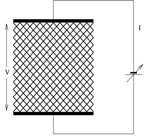
FIG. 20 A fuse model of size 100 \times 100 . Each bond is a fuse with a burn-out threshold t drawn from a probability distribution p(t) .
