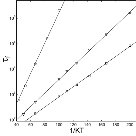
FIG. 46 Failure time \tau_f of an heterogeneous bundle ( KT_d \neq 0 ) in creep test. The life time \tau_f is plotted as a function of 1/KT at x_0 = 0.45 . Different symbols correspond to different values of KT_d : (Circle) KT_d = 0 ; (triangle) KT_d = 0.02 ; (box) KT_d = 0.04 . Adapted from Ciliberto et al. (2001).
