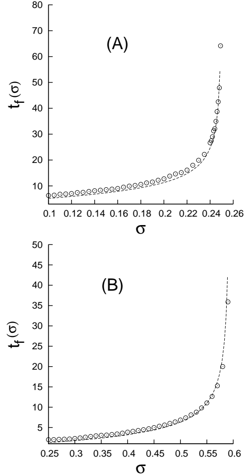
FIG. 12 Simulation results with pre-critical stress for (A) the uniform threshold distribution (Eq. 1), and (B) the Weibull distribution (2) with index 5. The graphs are based on 10000 samples with N = 10^6 fibers in each bundle. Open circles represent simulation data and the dotted lines are the theoretical estimates, Eq. (101) in (A) and Eq. (111-112) in (B).
