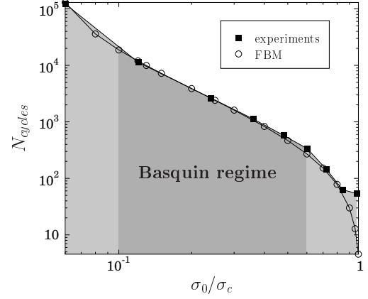
FIG. 55 Number of cycles at catastrophic failure, N_f as a function of load amplitude \sigma_0/\sigma_c . The two curves show experimental and fiber bundle model data respectively. From Kun et al. (2007).
