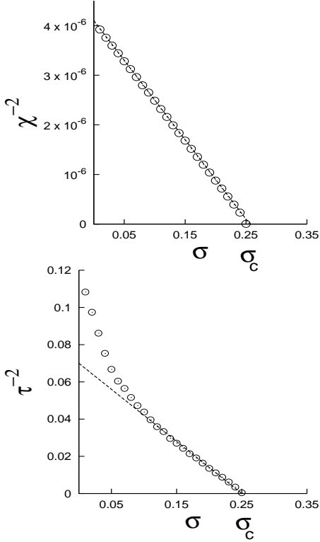
FIG. 56 Variation of \chi^{-2} and \tau^{-2} with applied stress for a bundle having N = 50000 fibers. Uniform distribution of fiber thresholds is considered and averages are taken over 1000 sample. The dotted straight lines are the best linear fits near the critical point.
