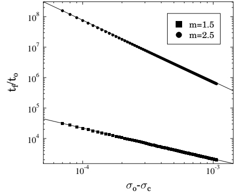
FIG. 52 Lifetime t_f as a function of the distance from the critical point, \sigma_o - \sigma_c , for two different values of the parameter m . The number of fibers in the bundle is N = 10^7 . From Kun et al. (2003).
