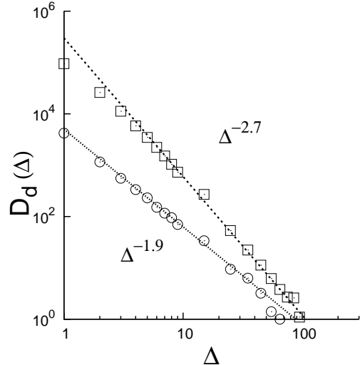
FIG. 23 The power dissipation avalanche histogram D_d(\Delta) for the fuse model. The slopes of the two straight lines are -2.7 and -1.9 , respectively. The circles show the histogram of avalanches recorded after 1000 fuses has blown, whereas the squares show the histogram recorded after 2090 fuses have blown. This is close to catastrophic failure.
