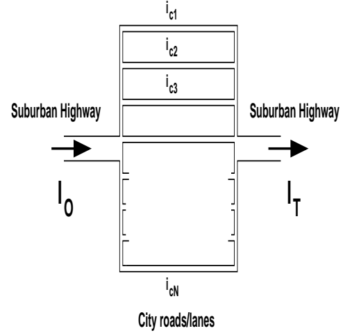
FIG. 66 The highway traffic current I_O gets fragmented into uniform currents i in each of the narrower roads and the roads having threshold current i_{c_n} \leq i get congested or blocked. This results in extra load for the uncongested roads. We assume that this extra load per uncongested roads gets equally redistributed and gets added to the existing load, causing further blocking of some more roads.
