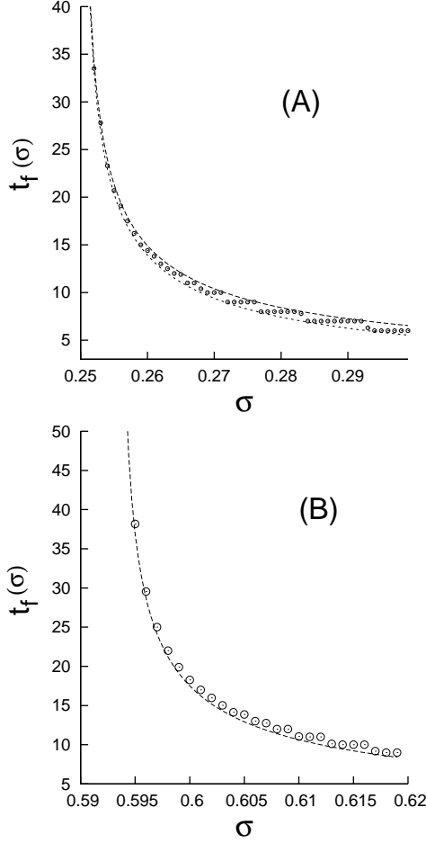
FIG. 10 Simulation results with post-critical stress for (A) the uniform threshold distribution (Eq. 1), and (B) the Weibull distribution (Eq. 2) with index 5. The graphs are based on 10000 samples with N = 10^6 fibers in each bundle. Open circles represent simulation data and dashed lines are the theoretical estimates Eq. (82), Eq. (83) in (A) and Eq. (92) in (B).
