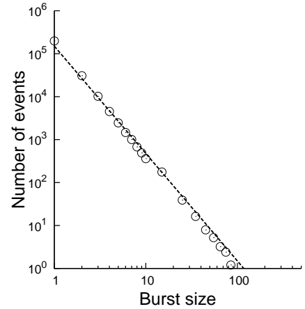
FIG. 43 Burst distribution for 128 \times 128 , e = 100 . The slope of the straight line is -2.5 .
