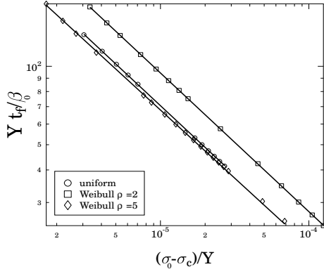
FIG. 50 The behavior of the time to failure t_f for uniform and Weibull distributions with two different Weibull index for the ELS case. All the three curves are parallel to each other on a double logarithmic plot with an exponent close to 0.5, in agreement with the general result Eq. (288). From Hidalgo et al. (2002).
