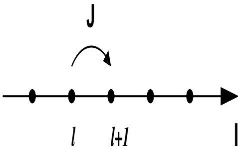
FIG. 67 The transport current I in the one dimensional lane or road is possible if, say, the l -th site is occupied and the (l + 1) -th site is vacant. The inter-site hopping probability is indicated by J .
