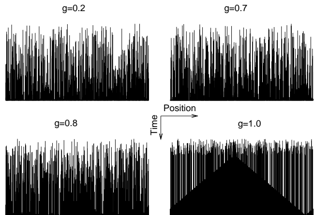
FIG. 34 Space time diagram of breaking sequences of the interpolating fiber bundle model of Pradhan et al. (2005). Black lines represent broken fibers and white regions are unbroken parts of the bundle. As the interpolation parameter g is increased, there is increasing localization of the failing fibers.
