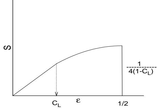
FIG. 13 The stress-strain curve for an ELS bundle having uniform fiber strength distribution with a low cutoff C_L = 0.2 .
