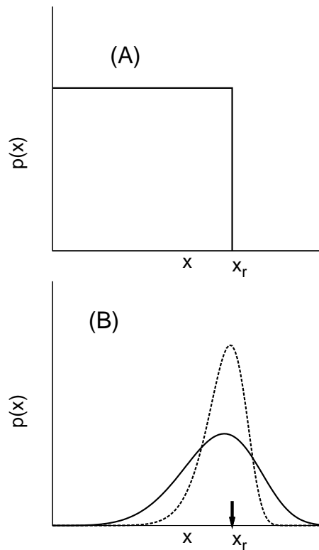
FIG. 2 The uniform distribution (A) and the Weibull distribution (B) with \rho = 5 (solid line) and \rho = 10 (dotted line).
