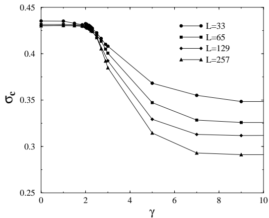
FIG. 35 Strength at failure, \sigma_c as a function of \gamma in the variable range fiber bundle of Hidalgo et al. (2002).
