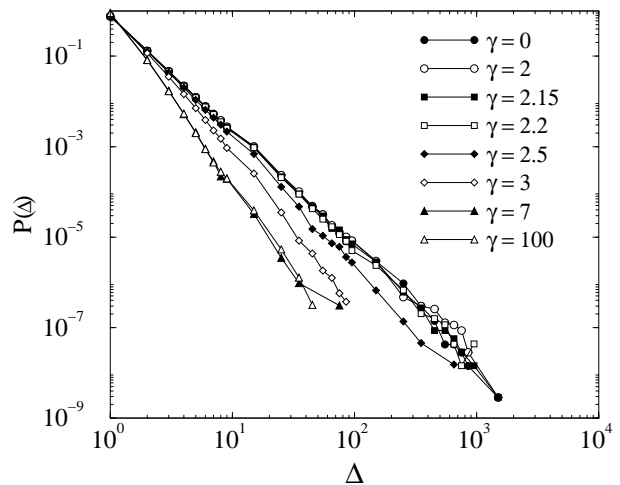
FIG. 37 Burst size distribution for different range exponents \gamma in the variable range fiber bundle of Hidalgo et al. (2002). The data points where \gamma \leq 2.0 can be fitted to a power law with exponent \xi = 5/2 . For larger \gamma , the slope becomes steeper and resembling the behavior seen in the local load-sharing model, see Fig. 31.
