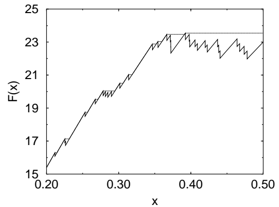
FIG. 15 The solid curve indicates the total force F(x) as a function of x . However, when our control parameter is F rather than x , the system will follow the dotted line, Eq. (138). The bursts are the horizontal parts of F_{ph}(x) . Here N = 100 .
