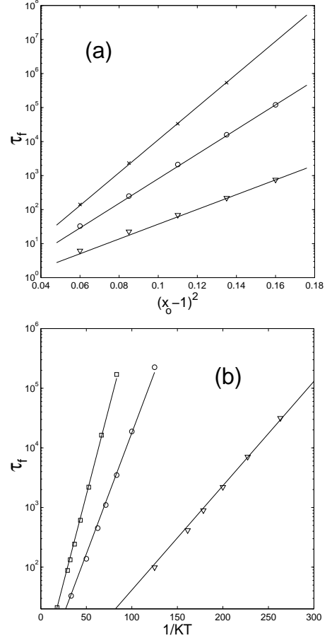
FIG. 45 Failure time \tau_f of an homogeneous bundle ( KT_d = 0 ) in a creep test. (a) \tau_f as a function of the normalized force (1 - x_0)^2 for several values of thermal noise variance KT : (cross) KT = 0.0045 ; (circle) KT = 0.006 ; (triangle) KT = 0.01 . (b) \tau_f as a function of 1/KT for several values of x_0 : (box) x_0 = 0.45 ; (circle) x_0 = 0.54 ; (triangle) x_0 = 0.7 . Continuous lines in (a) and (b) are the fits with Eq. (259) and Eq. (260), respectively. Adapted from Ciliberto et al. (2001).
