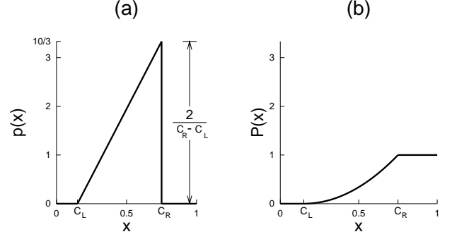
FIG. 4 (a) The density function p(x) and (b) the cumulative distribution P(x) of random fiber strengths x distributed with linearly increasing density in the interval [C_L, C_R] . In the particular instance shown in the figure C_L = 0.15 and C_R = 0.75 .
