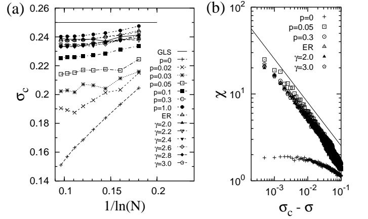
FIG. 65 (a) The system size ( N ) dependence of critical points ( \sigma_c ) for various networks with N = 2^8, 2^9, \dots, 2^{15} vertices. (b) The susceptibility for the networks with N = 2^{14} . p and \gamma are the rewiring probability in the WS networks and the exponent of degree distribution P(k) \sim k^{-\gamma} respectively. The data points are obtained from the averages over 10^4 ( 10^3 for N = 2^{15} ) ensembles. From Kim et al. (2005).
