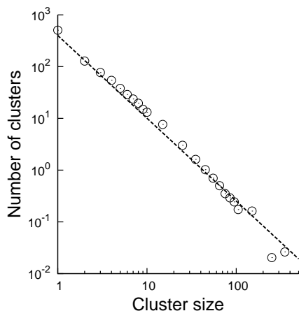
FIG. 44 Area distribution of zones where glue has failed for systems of size 128 \times 128 and elastic constant e = 10 . The straight line is a least square fit and indicates a power law with exponent -1.6 .
