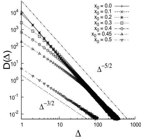
FIG. 60 The avalanche size distributions for different values of x_0 in ELS model with uniform fiber strength distribution. Here bundle size N = 50000 and averages are taken over 10000 sample. Two power laws (dotted lines) have been drawn as reference lines to compare the numerical results.
