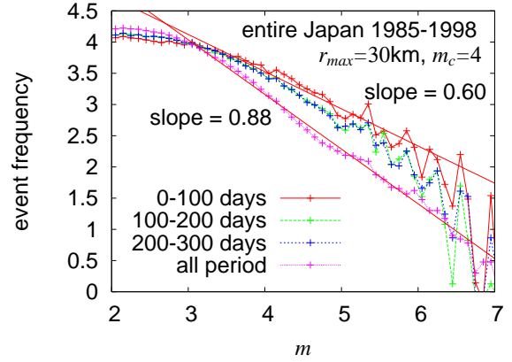
FIG. 61 Crossover signature in the local magnitude distributions of earthquakes in Japan. The exponent of the distribution during 100 days before a mainshock is about 0.60, much smaller than the average value 0.88. From Kawamura (2006).
