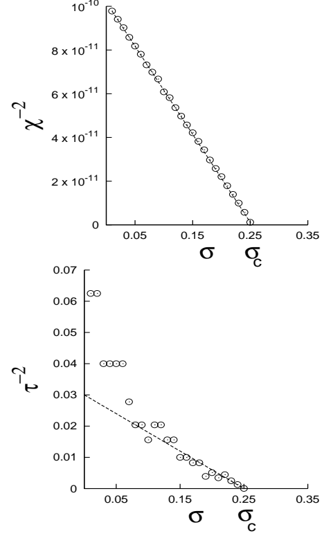
FIG. 57 Variation of \chi^{-2} and \tau^{-2} with applied stress for a single bundle having N = 10000000 fibers with uniform distribution of fiber thresholds. Straight lines represent the best linear fits near the critical point.
