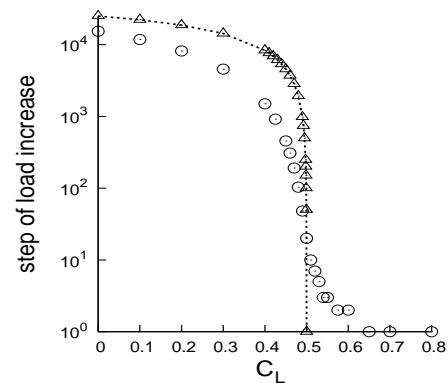
FIG. 14 The number of steps of load increase (till final failure) is plotted against C_L for a ELS model having 50000 fibers. The dotted line represents the analytic form (eqn. 136), triangles are the simulated data for a strictly uniform strength distribution, and the circles represent the data (averages are taken for 5000 samples) for a uniform distribution on average.
