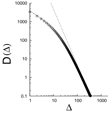
FIG. 27 Avalanche size distribution for the Weibull distribution (2) with index 5. Open circles represent simulation data, dashed lines are analytic expressions (Eq. 213) and dotted line is the asymptotic power law with exponent -3 . The load is increased in steps of \delta = 20 . The figure is based on 10000 samples of bundles with N = 10^6 fibers.
