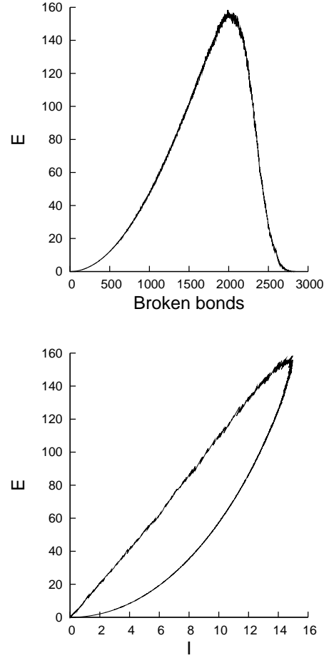
FIG. 22 Power dissipation E as a function of the number of broken bonds (upper) and as a function of the total current I flowing in the fuse model (lower).
