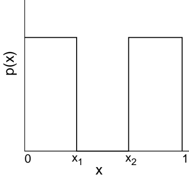
FIG. 24 Mixed uniform distribution.
