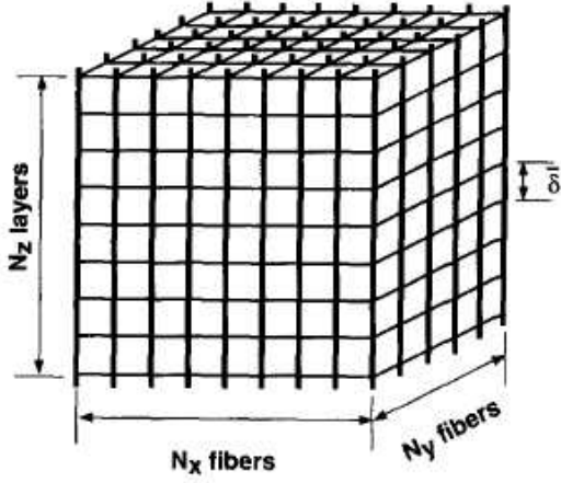
FIG. 64 The discretization of a three-dimensional unidirectional fiber reinforced composite used by Zhou and Curtin (2001).
