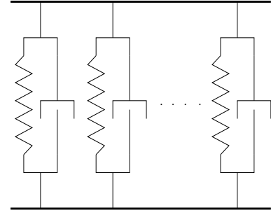
FIG. 49 The viscoelastic fiber bundle: intact fibers are modeled by Kelvin-Voigt elements which consists of a spring and a dashpot in parallel. From Kun et al. (2003).
