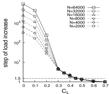
FIG. 32 Numerical estimate of the upper bound of C_L in LLS model: For C_L \geq 0.5 the average step values go below 1.5, i.e., the bundle fails at one step in most of the realizations.
