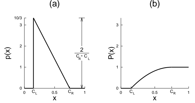
FIG. 6 (a) The density function p(x) and (b) the cumulative distribution P(x) of fiber strengths x distributed with linearly decreasing density in the interval [C_L, C_R] . Similar to the cases shown in Fig. 4 we have C_L = 0.15 and C_R = 0.75 in this example also.
