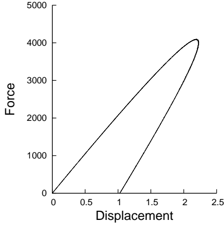
FIG. 40 Force-displacement curve, 128 \times 128 systems with e = 10 .
