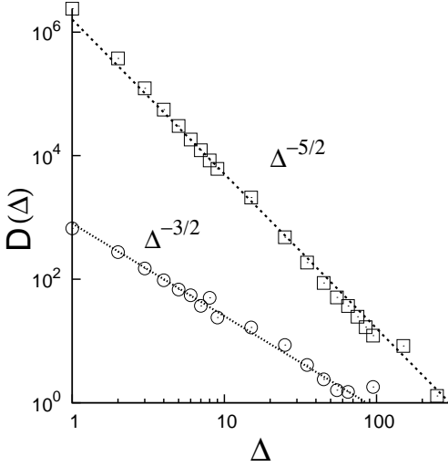
FIG. 19 The distribution of bursts for the uniform threshold distribution for a single fiber bundle with N = 10^7 fibers. Results with x_0 = 0 , i.e., when all bursts are recorded, are shown as squares and data for bursts near the critical point ( x_0 = 0.9x_c ) are shown by circles.
