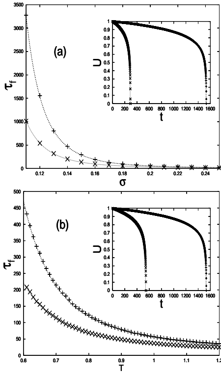
FIG. 47 The simulation results showing variation of average failure time \tau_f against (a) external stress \sigma and (b) against noise T ( K = 1 here), for a homogeneous bundle containing N = 10^5 fibers. The insets show the variation of the fraction U of unbroken fibers with time t for different T values [1.2 (cross) and 1.0 (plus)] in (a) and different \sigma values [0.15 (cross) and 0.12 (plus)] in (b). The dotted and dashed lines represent the theoretical result Eq. (277).
