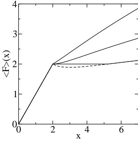
FIG. 17 The macroscopic bundle strength \langle F \rangle(x) for the distribution (Eq. 177), with x_0 = 2x_r , and for \alpha_0 = \frac{1}{3} (upper curve), \frac{1}{2} (middle curve), and \frac{2}{3} (lower curve). The broken part of the \alpha_0 = 2/3 -curve is unstable and the macroscopic bundle strength will follow the solid line.
