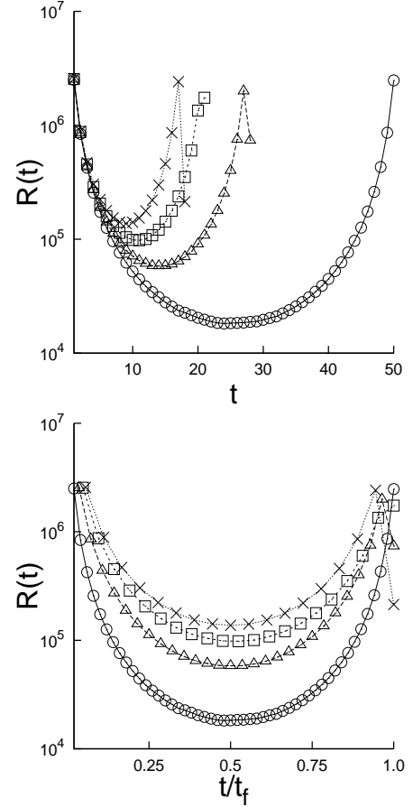
FIG. 59 The breaking rate R(t) vs. step t (upper plot) and vs. the rescaled step variable t/t_f (lower plot) for the uniform threshold distribution for a bundle of N = 10^7 fibers. Different symbols are used for different excess stress levels \sigma - \sigma_c : 0.001 (circles), 0.003 (triangles), 0.005 (squares) and 0.007 (crosses).
