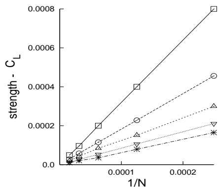
FIG. 33 The strength - C_L is plotted against 1/N for different C_L values: 0.3 (square), 0.35 (circle), 0.4 (up triangle), 0.45 (down triangle), 0.5 (star). All the straight lines approach 0 value as N \rightarrow \infty .
