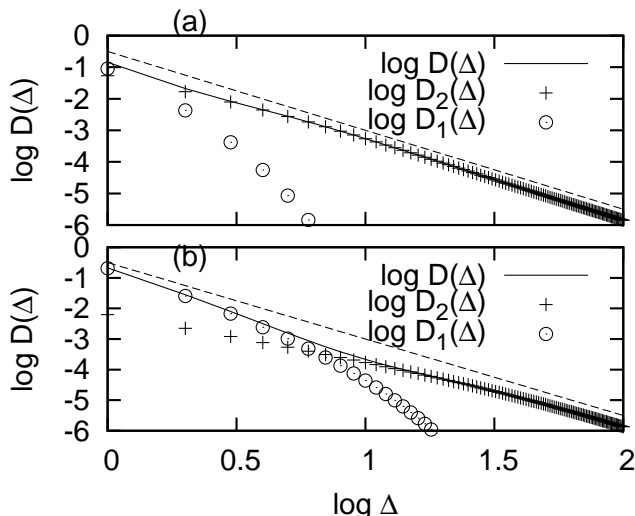
FIG. 25 Total avalanche size distribution D(\Delta) , D_1(\Delta) and D_2(\Delta) obtained by numerical integration of Eqs. (200) and (201). Figure (a) corresponds to x_1 = 0.08 , x_2 = 0.28 and f = 0.1 and Figure (b) to x_1 = 0.25 , x_2 = 0.42 and f = 0.3 . As x_2 \rightarrow 0.5 , the nonuniversal region increases in the small \Delta region, whereas \Delta \propto \Delta^{-5/2} for large \Delta . The dotted line has a slope of -5/2 . From Divakaran and Dutta (2007a).
