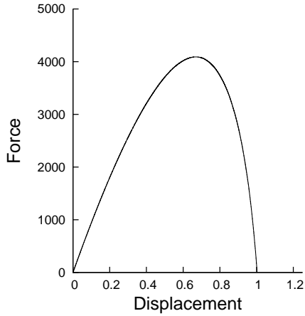
FIG. 41 Force-displacement curve, 128 \times 128 systems with e = 100 .
