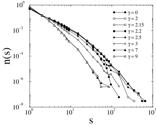
FIG. 38 Size distribution of clusters of broken bonds at collapse in the variable range fiber bundle of Hidalgo et al. (2002). There is no evident power law behavior.
