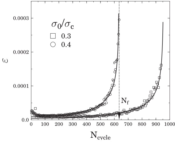
FIG. 54 Deformation \varepsilon as a function of number of cycles N_{cycle} , showing both experimental data and theoretical curves based on the fiber bundle model. From Kun et al. (2007).
