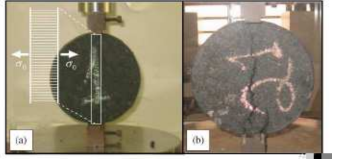
FIG. 53 Asphalt samples set up for experimental testing of fatigue failure. Figure (a) shows how fatigue failure under these experimental conditions are modeled using a fiber bundle model and (b) shows a post-failure sample. From Kun et al. (2007).
