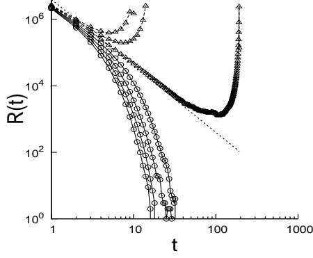
FIG. 58 Log-log plot of breaking-rate with step of load redistribution for 7 different stress values. Circles are for stresses below the critical stress and triangles are for stresses above the critical stress. The simulation has been performed for a single bundle with N = 10000000 fibers having uniform distribution of fiber thresholds. The dotted straight line has a slope -2 .
