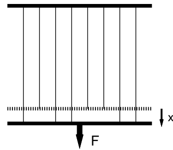
FIG. 1 A fiber bundle model having N parallel fibers. The original position of the rigid platform on which force has been applied, is indicated. All the fibers are assumed to have the same elastic constant (normalized to unity here) until breaking, while the breaking strength of these fibers are assumed to be randomly dispersed. As the bundle gets strained ( x > 0 ), some weaker fibers (having lower stress or strain capacity) fail, and the number of intact fibers decrease from its starting value N . Consequently, the stress on them (or the strain) increases due to the redistribution or transfer of loads from the failing fibers. Some of these fibers may fail further as they can not support this extra redistributed load. The process stops if there is no further failure, and the bundle will show non-linear elastic response (although each fiber has linear elastic behavior until breaking). Otherwise, the bundle fails when the stress concentration on the fibers (due to the dynamic stress redistribution) becomes so high that none of the fibers can withstand that.
