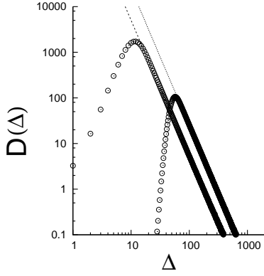
FIG. 26 Avalanche size distribution for the uniform threshold distribution (Eq. 1) when the load is increased in steps of \delta = 10 and \delta = 50 (upper curve). The dotted lines show the theoretical asymptotics (Eq. 208) for \delta = 10 and \delta = 50 . The figure is based on 10000 samples with N = 10^6 fibers in the bundle.
