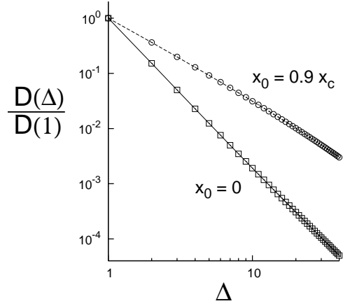
FIG. 18 The distribution of bursts for thresholds uniformly distributed in an interval (x_0, x_c) , with x_0 = 0 and with x_0 = 0.9x_c . The figure is based on 50 000 samples, each containing N = 10^6 fibers. The exponents of the distributions are \xi = 5/2 and \xi = 3/2 respectively.
