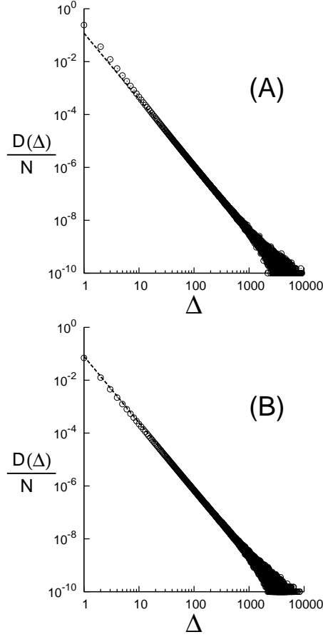
FIG. 16 The burst distribution D(\Delta)/N for the uniform distribution (A) and the Weibull distribution with index 5 (B). The dotted lines represent the power law with exponent \xi = 5/2 . Both figures are based on 20000 samples of bundles each with N = 10^6 fibers.
