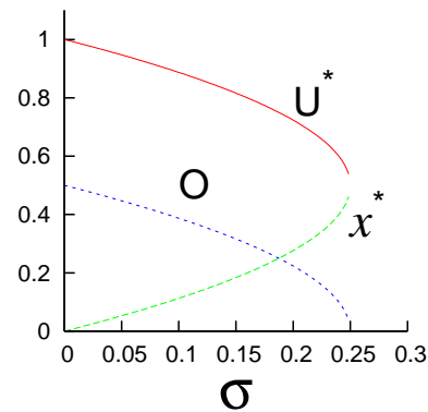
FIG. 3 Variation of effective stress ( x^* ), fraction of unbroken fibers ( U^* ) and the order parameter ( O ) with the applied stress \sigma for a bundle with uniform distribution (Eq. 1) of fiber strengths.
