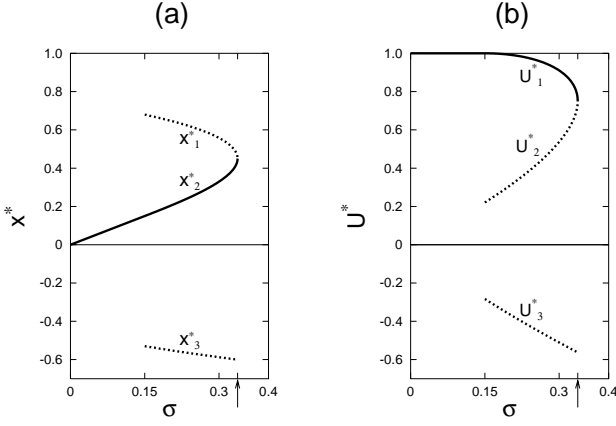
FIG. 5 The fixed points of (a) the redistributed stress, and (b) the surviving fraction of fibers for the distribution of fiber strengths shown in Fig. 4. In each part of the figure the curve for the stable fixed points is shown by a bold solid line and those for the unstable fixed points are shown by bold broken lines. We have C_L = 0.15 and C_R = 0.75 , so that \sigma_c = 0.3375 ; the position of the critical point is marked by an arrowhead. For \sigma \leq C_L the fixed points are trivial: since there are no broken fibers x^* = \sigma and U^* = U_0 = 1 .
