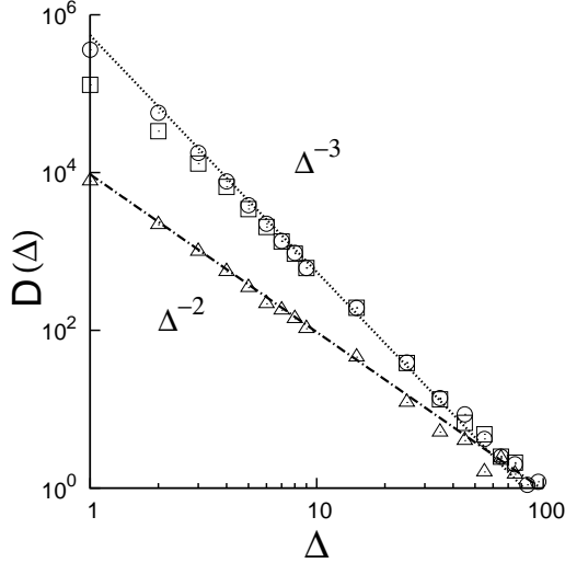
FIG. 21 The burst distribution based on 300 samples random fuse lattices of size 100 \times 100 . The threshold t are uniformly distributed on the unit interval. On the average, catastrophic failure sets in after 2097 fuses have blown. The circles denote the burst distribution measured throughout the entire breakdown process. The squares denote the burst distribution based on bursts appearing after the first 1000 fuses have blown. The triangles denote the burst distribution after 2090 fuses have blown. The two straight lines indicate power laws with exponents \xi = 3 and \xi = 2 , respectively.
