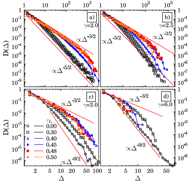
FIG. 39 Burst size distributions in the variable range fiber bundle model for different \gamma and \epsilon_L values: a) \gamma = 2.0 , b) \gamma = 2.5 , c) \gamma = 3.0 and d) \gamma = 6.0 . From Raischel et al. (2006).
